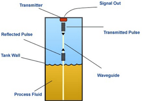
Guided Wave Radar System
